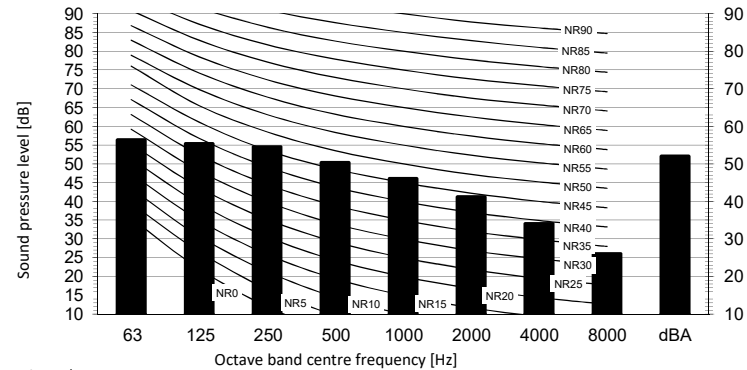
Cooling mode
