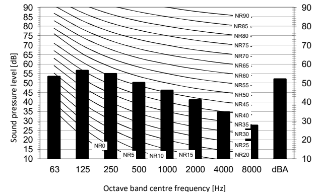
Heating mode
