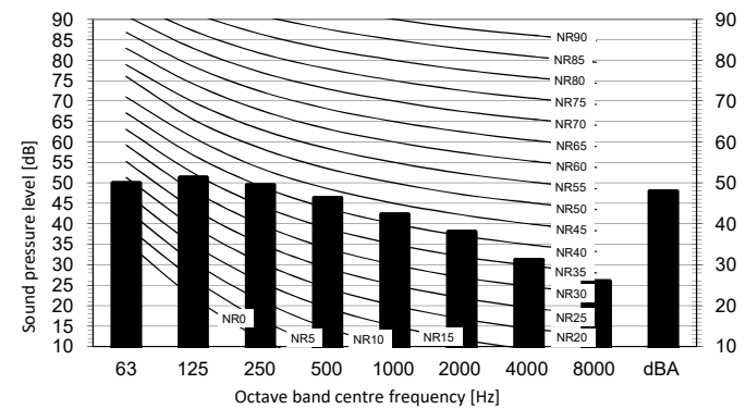
Heating mode
