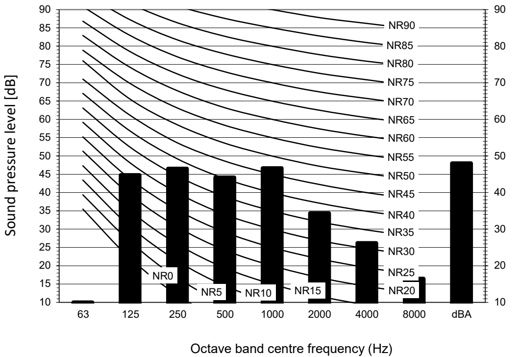
Heating mode
