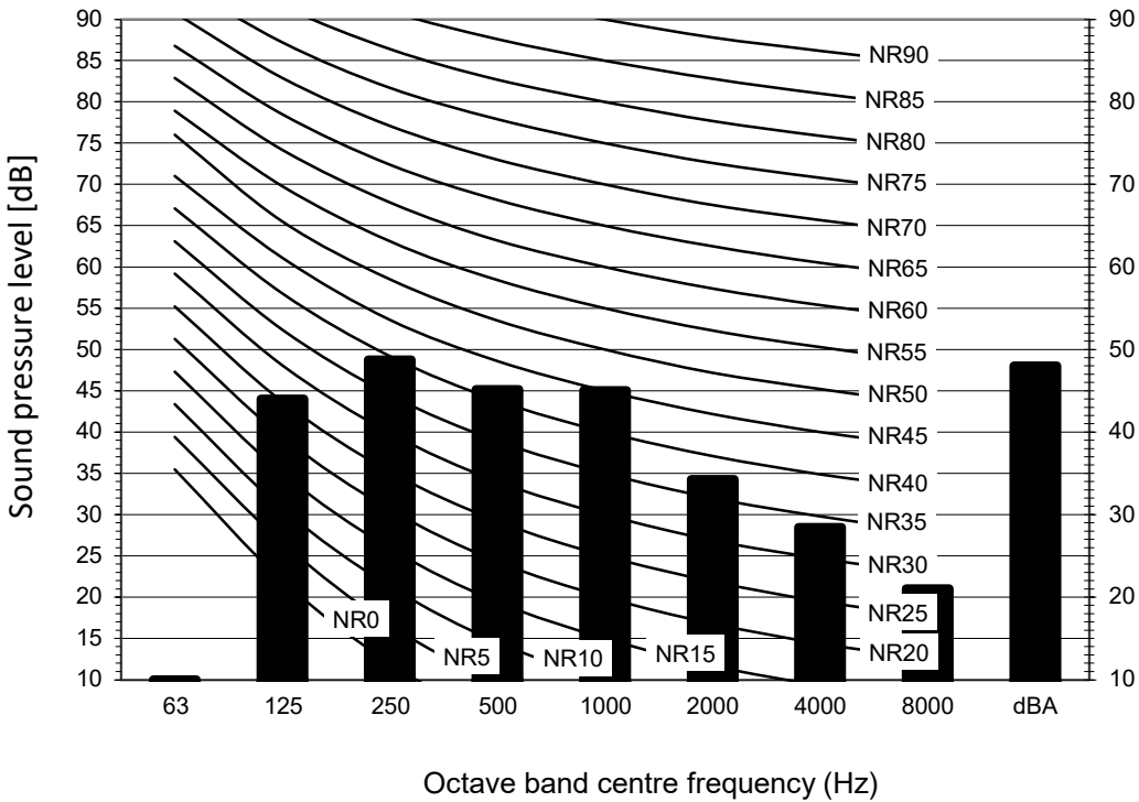
Cooling mode
