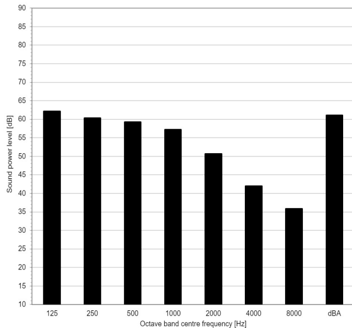
Cooling mode
