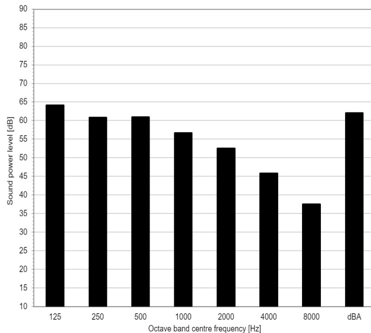
Heating mode
