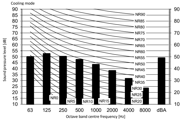
Cooling Total dB
