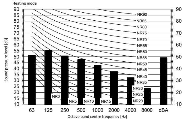
Heating Total dB
