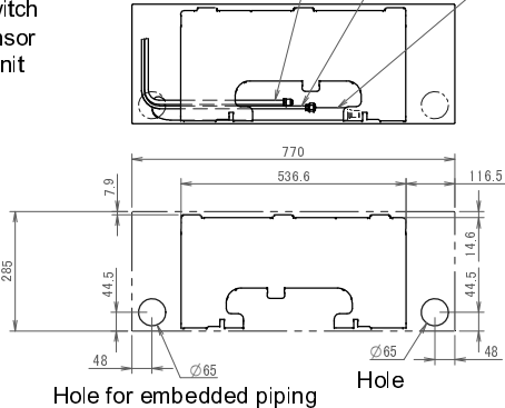
Standard location of holes in the wall
