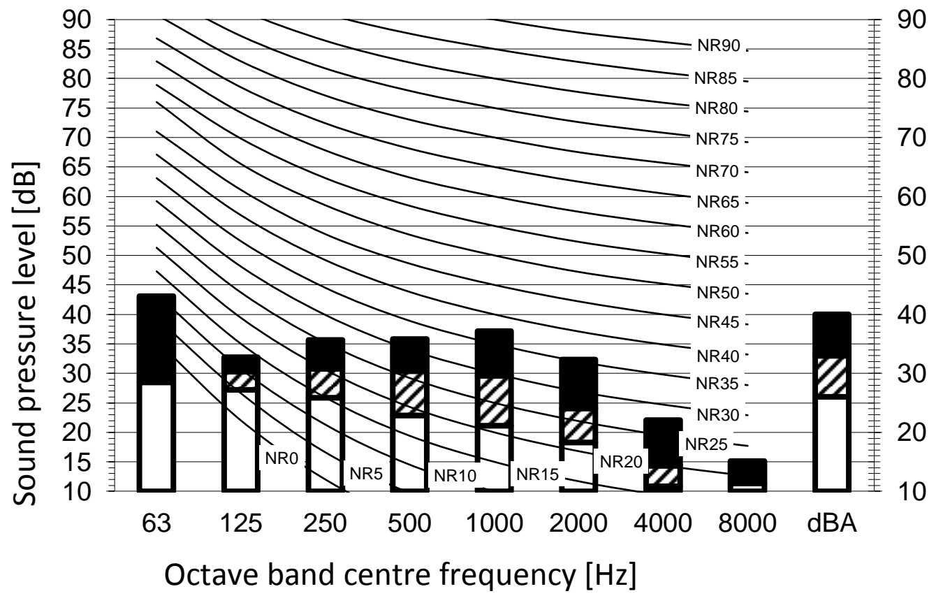
Cooling mode
