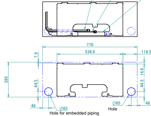
Standard location of holes in the wall
