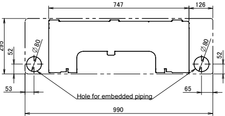
Standard location of holes in the wall
