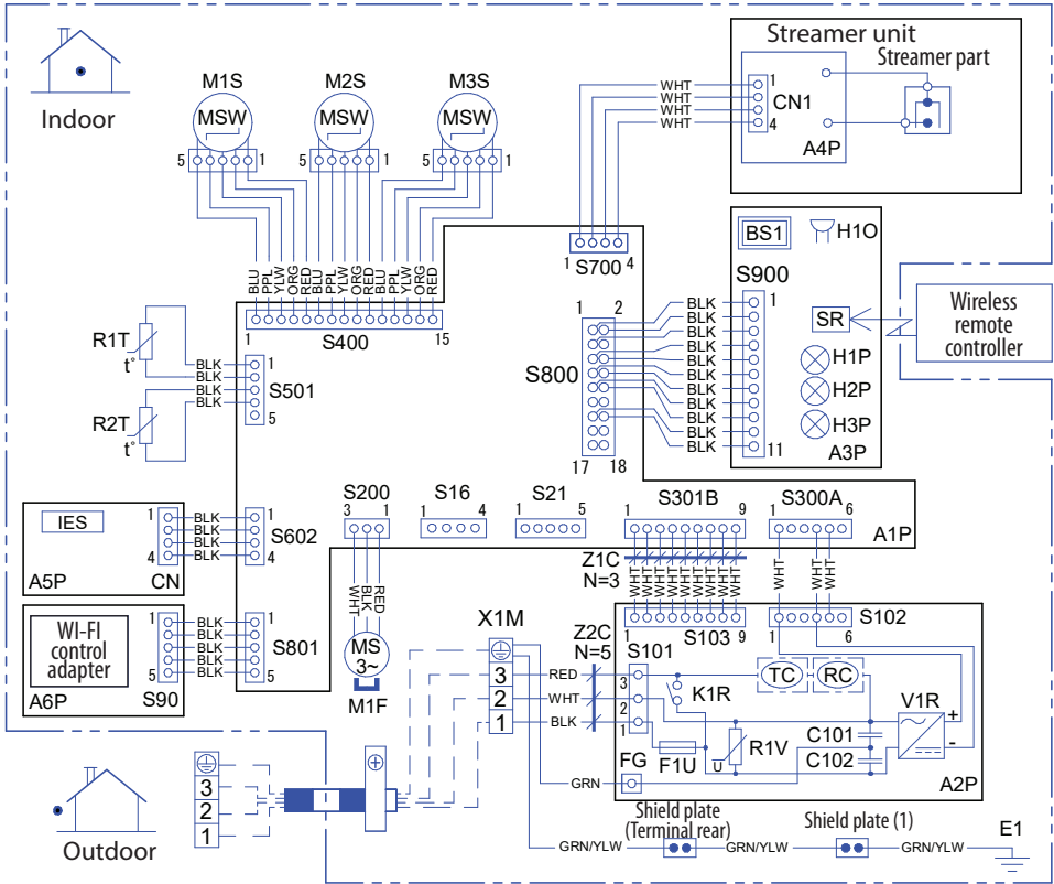
Wiring diagram
