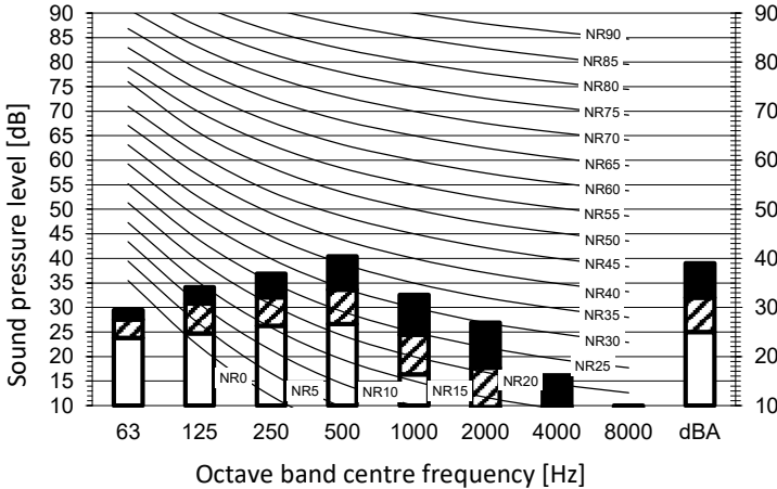
Cooling mode
