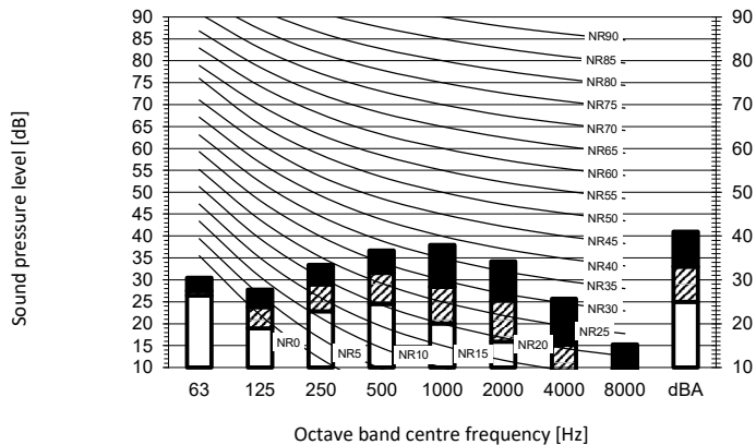
Cooling mode
