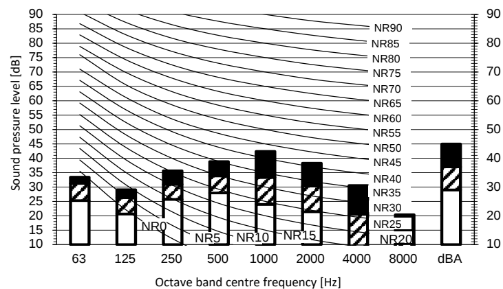
Heating mode
