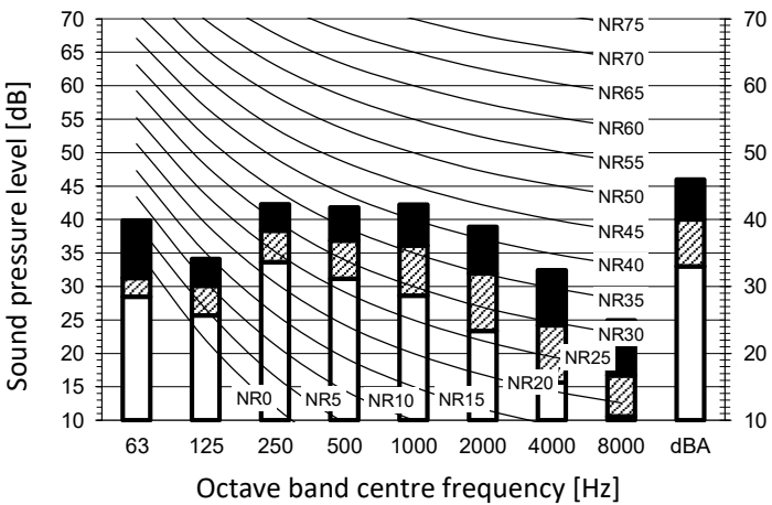
Cooling Total dB
