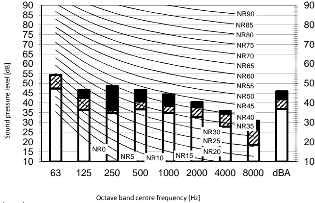
Cooling mode
