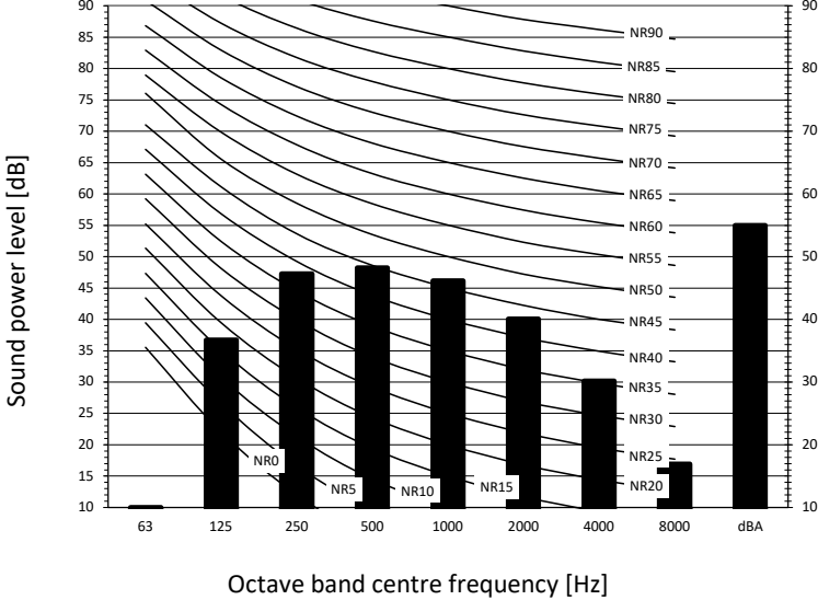
Heating mode
