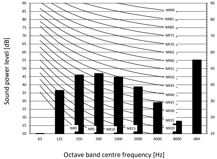
Cooling mode
