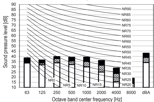
Cooling mode
