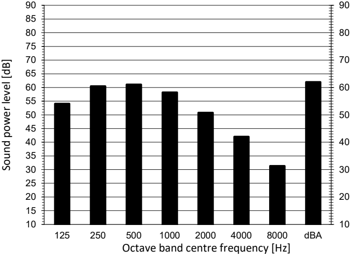
Heating mode
