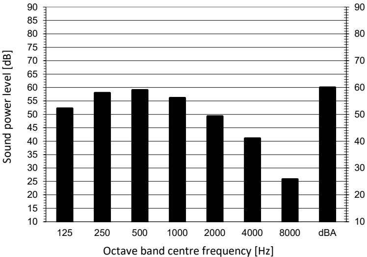
Cooling mode
