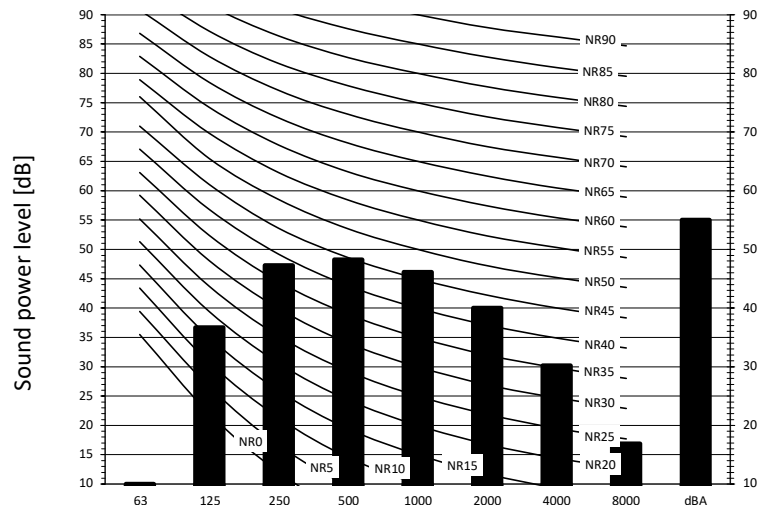
Heating mode
