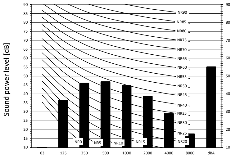
Cooling mode
