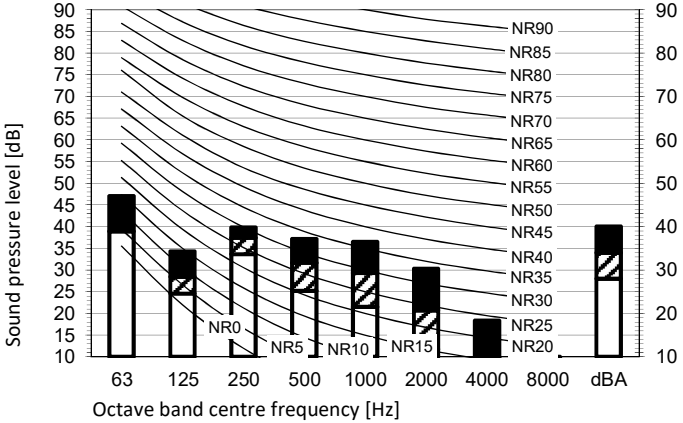
Heating mode
