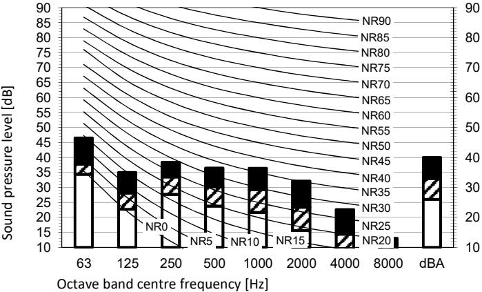
Cooling mode
