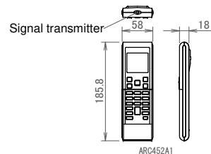
Wireless remote control
