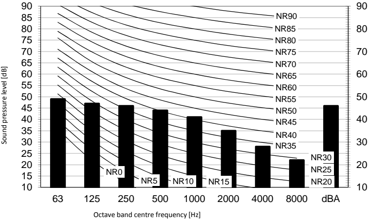
Cooling mode
