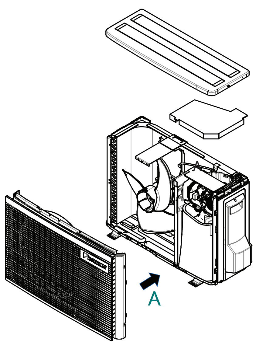
Disassembly of unit
