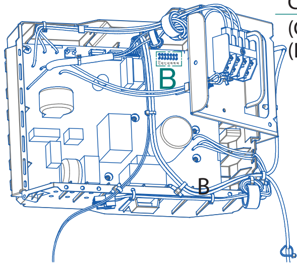
Arrow view A El. Compo. Assy
