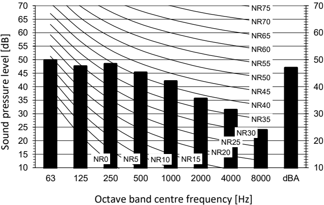
Heating mode
