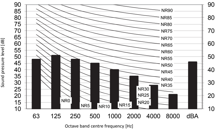
Cooling mode
