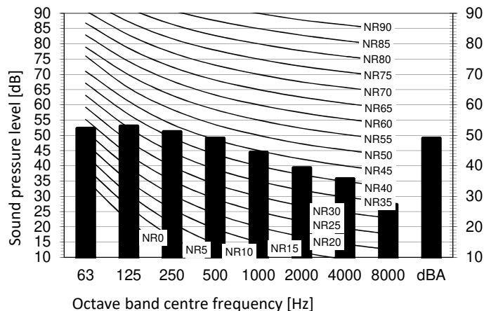
Cooling mode
