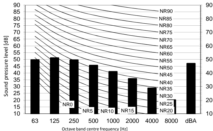
Cooling mode
