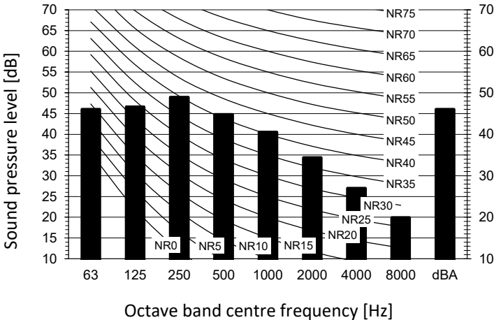
Cooling mode
