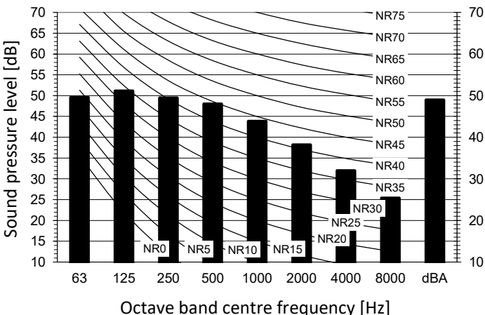
Heating mode
