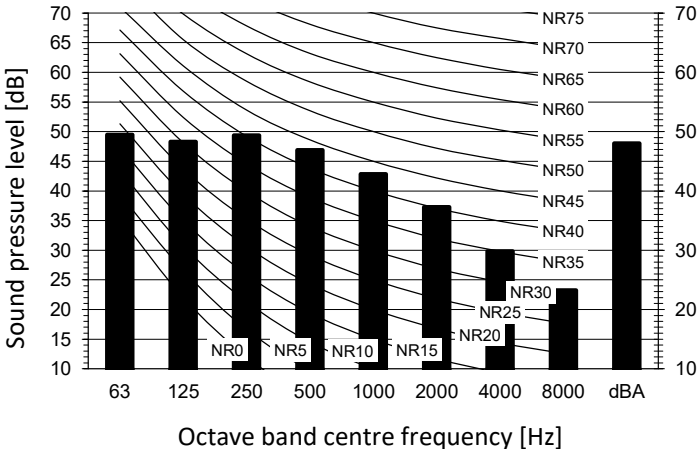
Cooling mode
