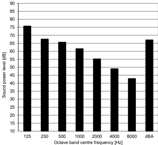
Heating mode
