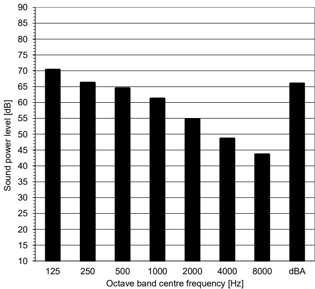
Cooling mode
