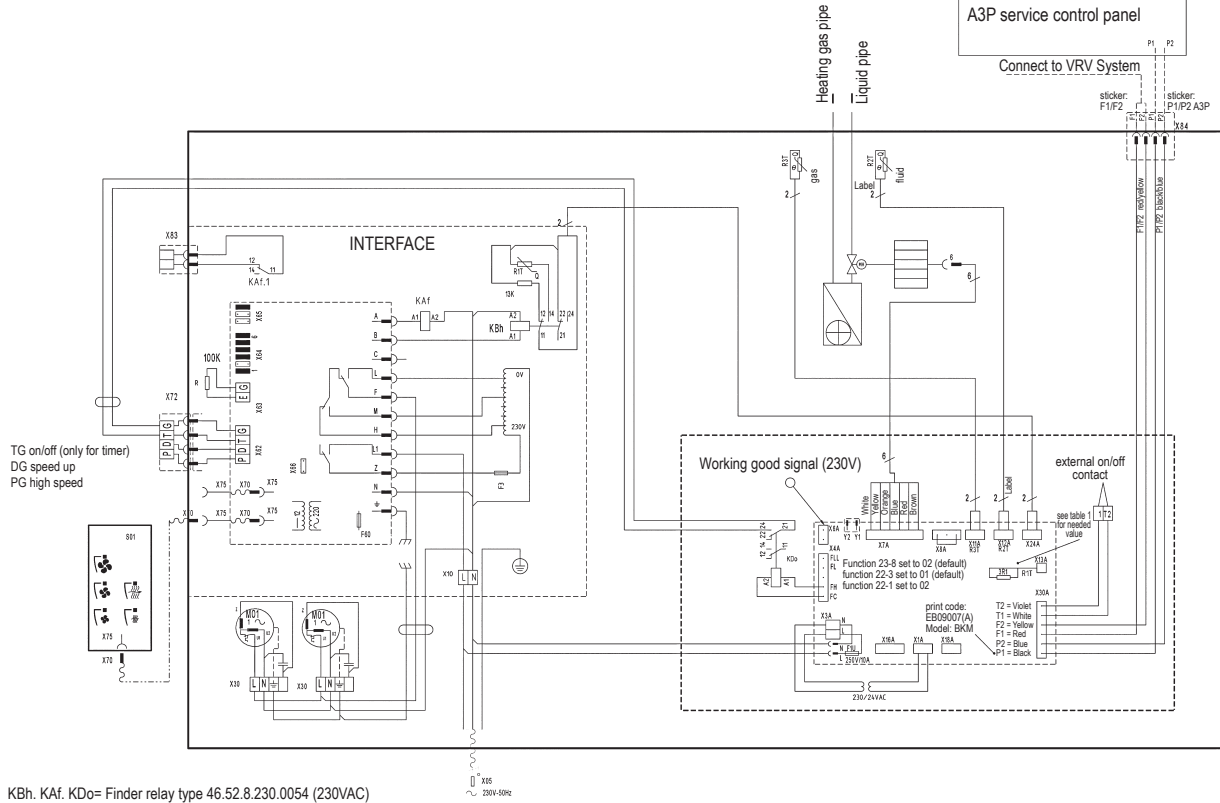
KBh. KA1. KD= Finder relay type 46.52.8.230.0054 (230VAC)
