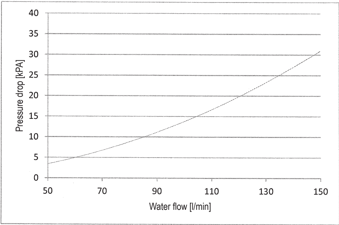
VRV4 Watercooled waterfilter flowing quantity characteristic
