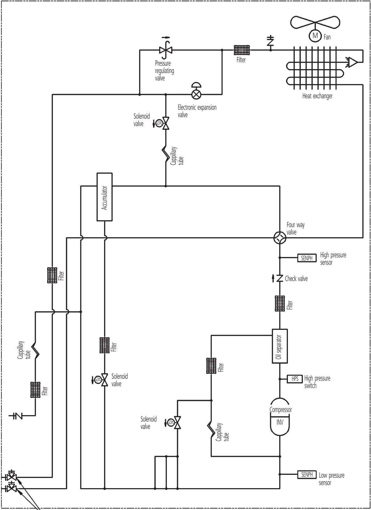
Stop valve (With service port on on-site piping side \varnothing 7.9\text{mm} flare connection)
