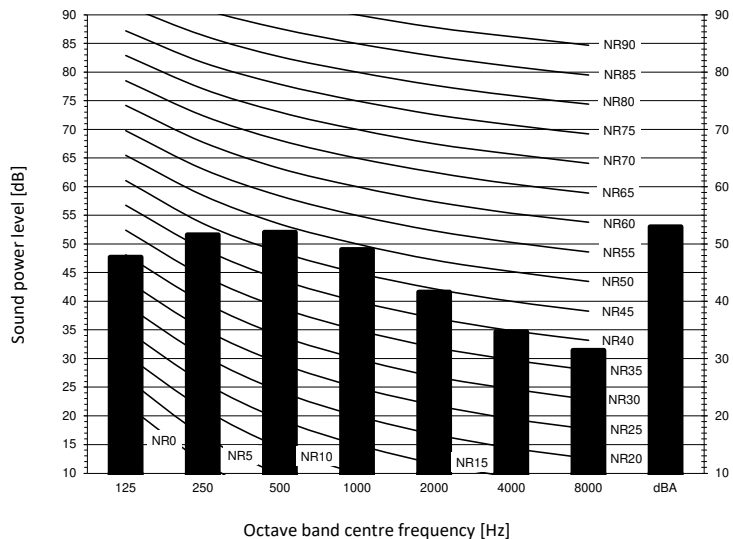
Cooling mode
