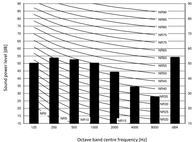
Heating mode
