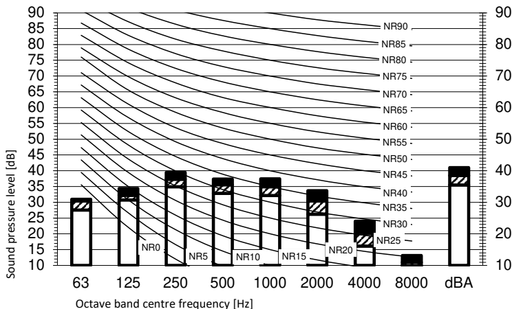
Cooling mode
