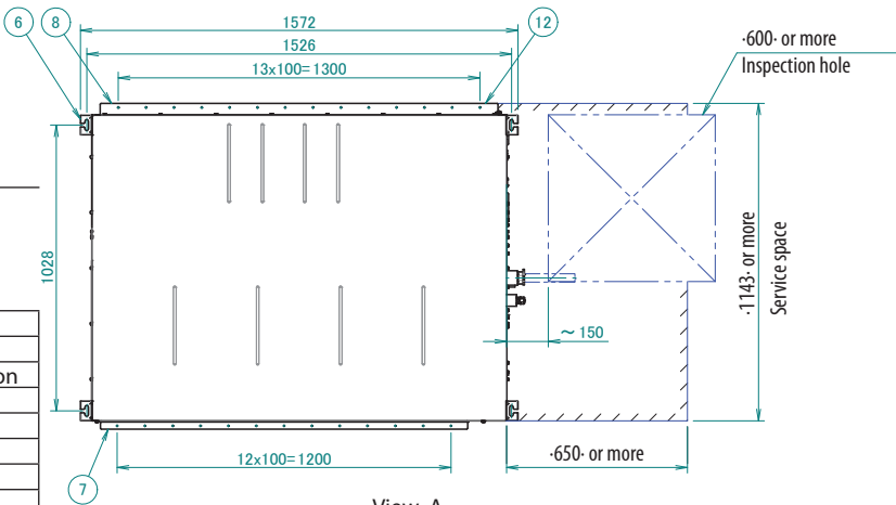
View -A-
