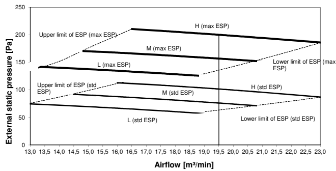
Fan characteristics (1)
