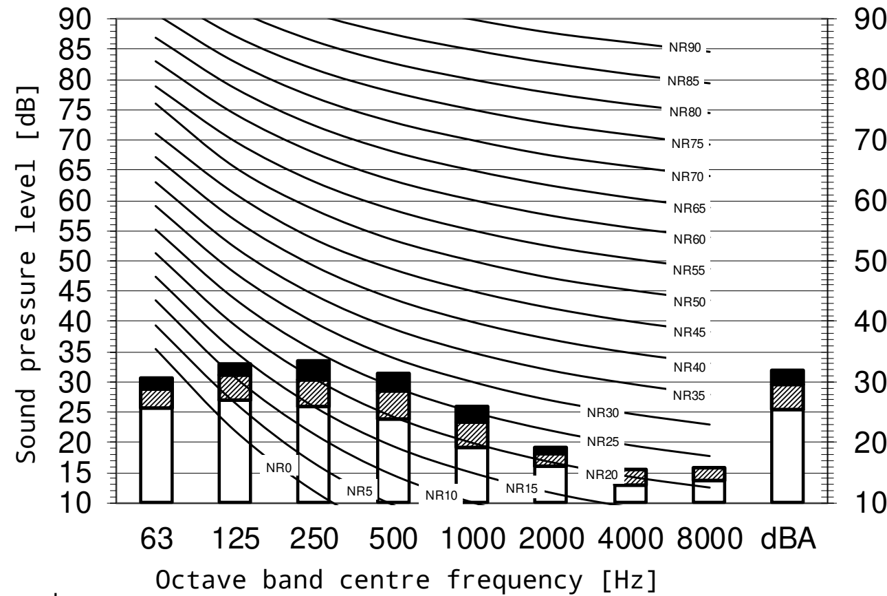
Cooling mode
