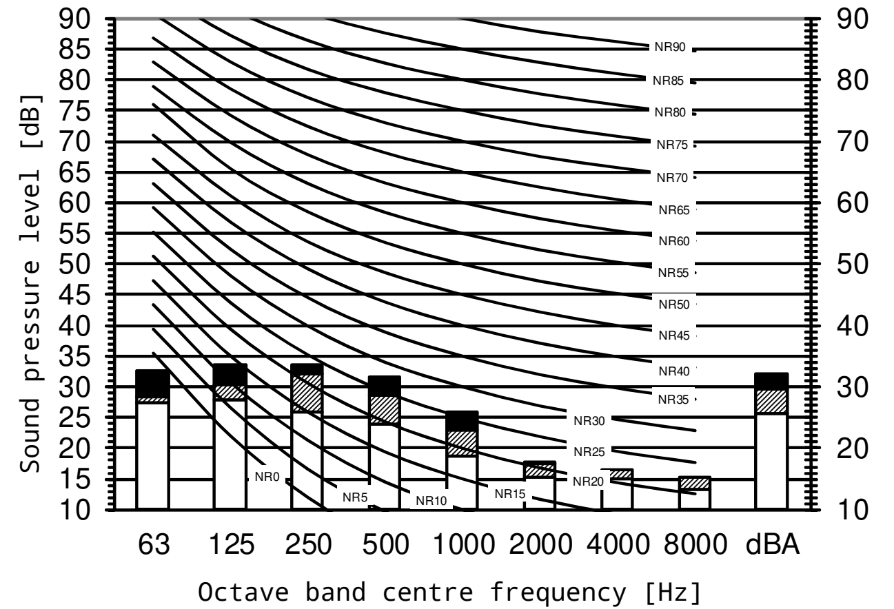
Heating mode
