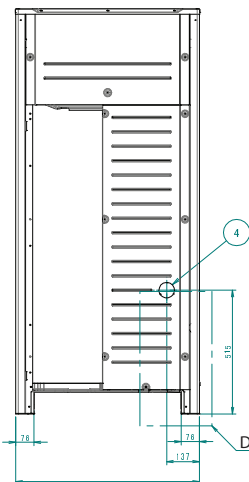
Detail A
