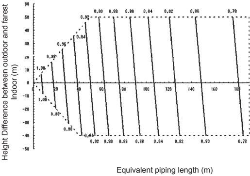
Correction ratio for cooling capacity
