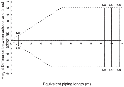
Correction ratio for heating capacity
