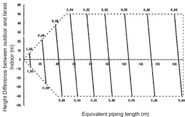
Correction ratio for cooling capacity
