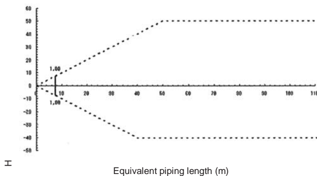
Correction ratio for heating capacity
