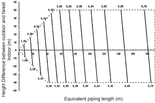
Correction ratio for cooling capacity
