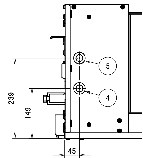
View A
