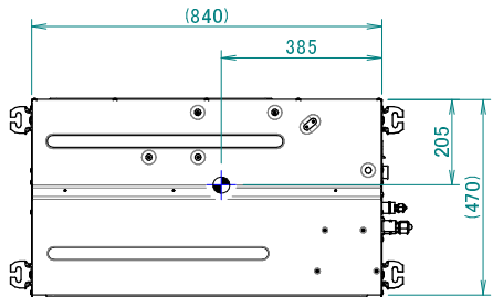
Indoor unit
