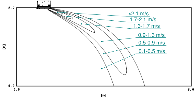
Air velocity distribution (cooling) Air flow direction: horizontal
