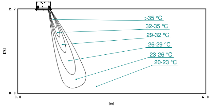
Air temperature distribution (heating) Air flow direction: vertical
