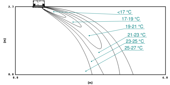
Air temperature distribution (cooling) Air flow direction: horizontal
