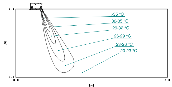
Air temperature distribution (heating)
