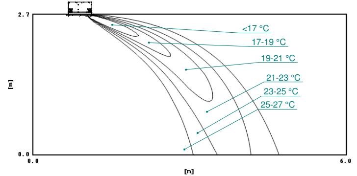
Air temperature distribution (cooling)
