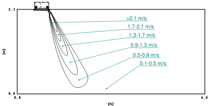
Air velocity distribution (heating)
