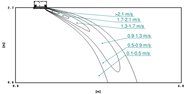
Air velocity distribution (cooling)
