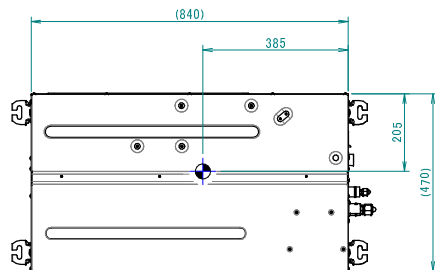
Indoor unit
