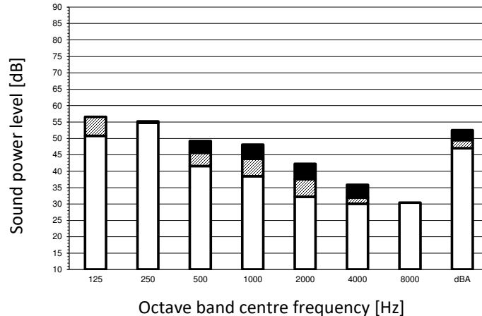
Heating mode
