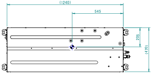
Indoor unit
